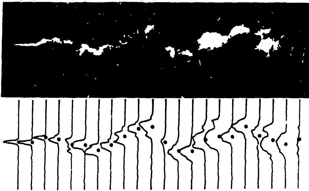
Fig. 1 4 Instantaneous and time-averaged photograph of the smoke plume with vertical profiles of the optical density and centroid positions over the region 0 < x < 3 m.
