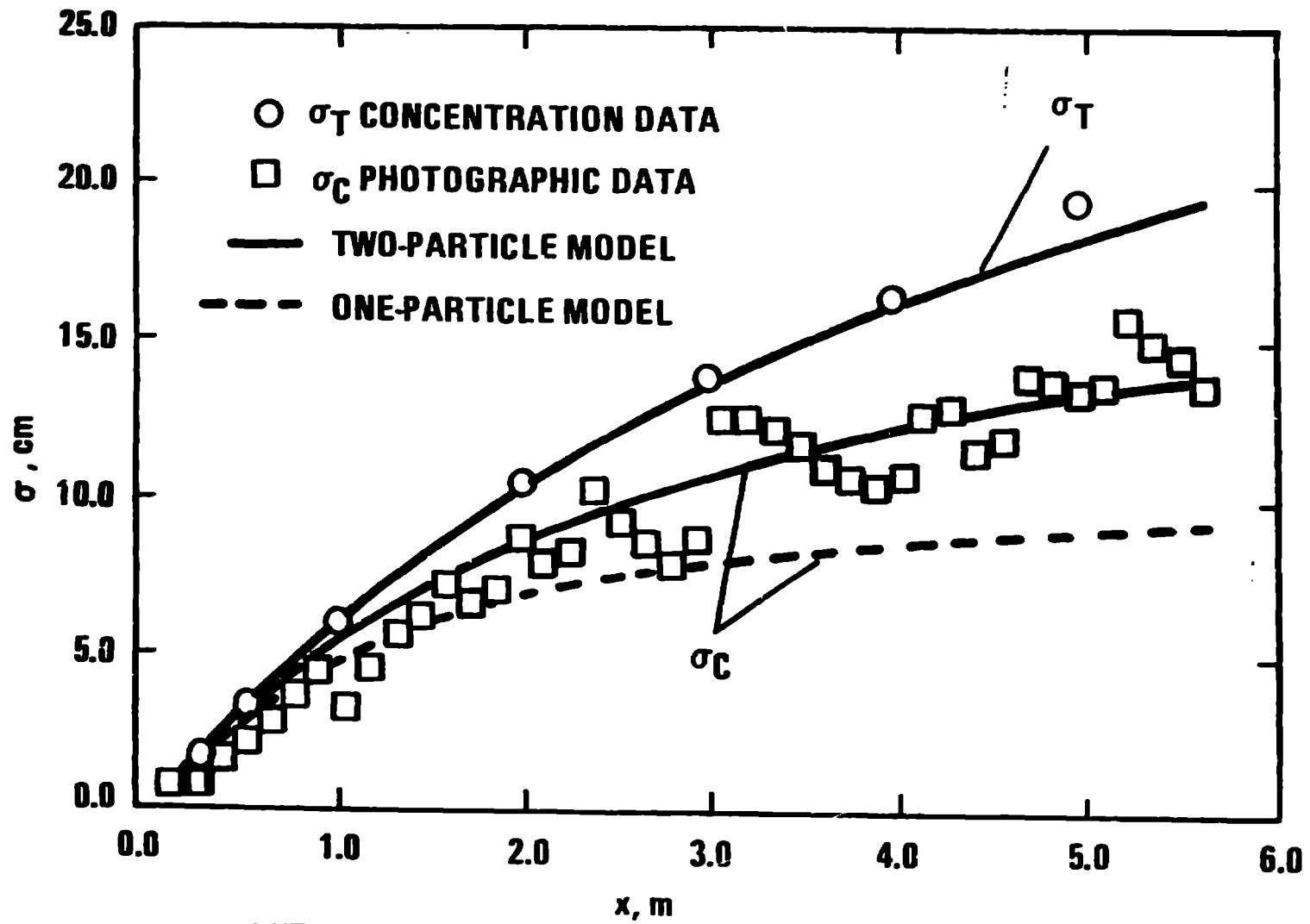
5 Fig. 10 Comparison of concentration and photographic data to one-particle and two-particle Monte Carlo simulations.
